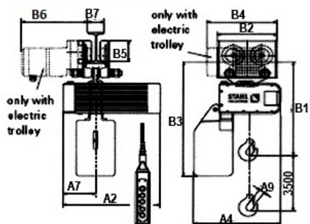
Chain hoist with trolley
