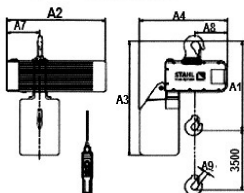
Chain hoist with hook suspension
