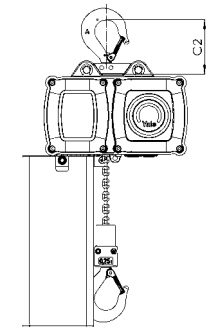
CPV/CPVF with suspension hook, 125 - 2500 kg
