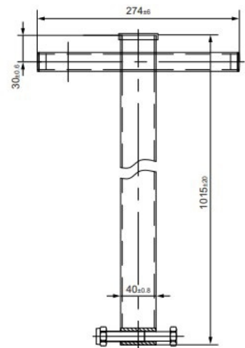
HAND LEVER
