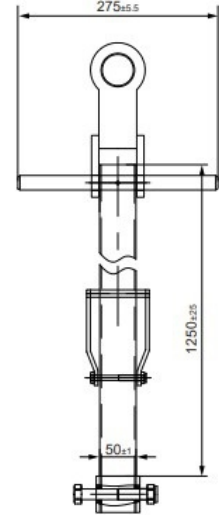
HAND LEVER
