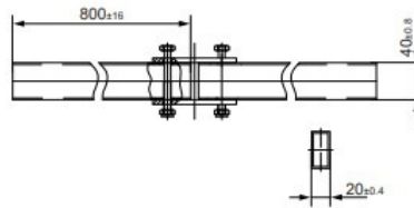
CONNECTOR BAR
