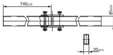
CONNECTOR BAR
