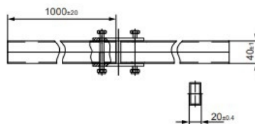
CONNECTOR BAR
