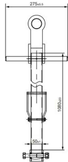
HAND LEVER
