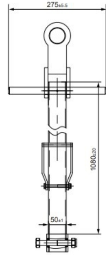
HAND LEVER
